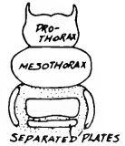
Fig. 399. Dorsal aspect of thorax.
